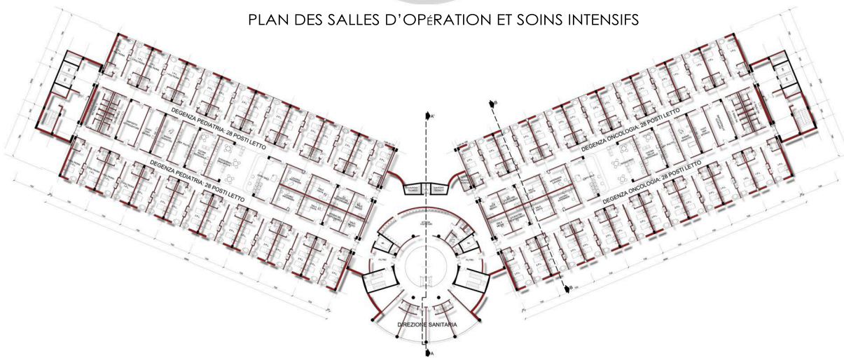
PLAN TYPE
