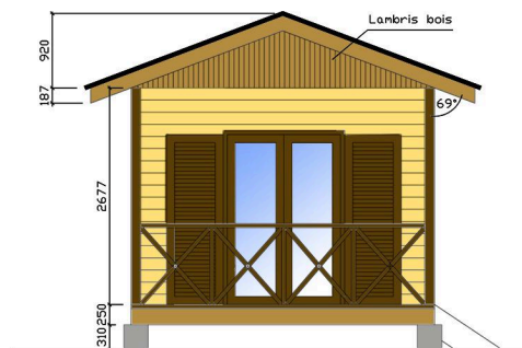
FAÇADE PRINCIPALE
