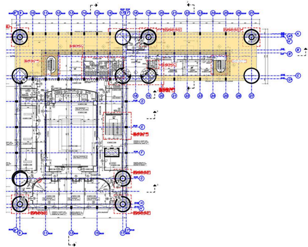
MEZZANINE PLAN
