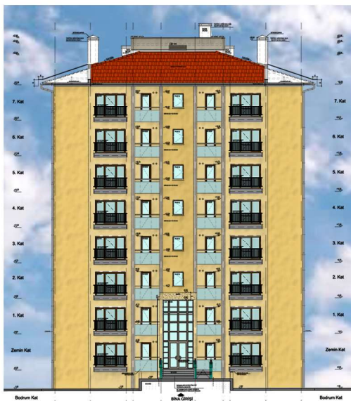
MAIN FACADE
