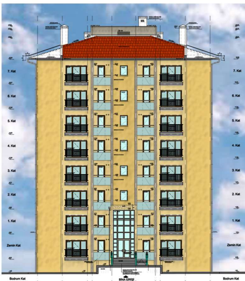
FAÇADE PRINCIPALE
