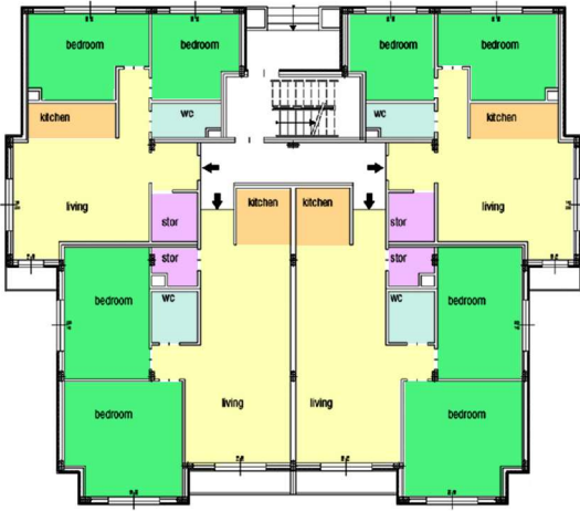
TYPE FLOOR PLAN
