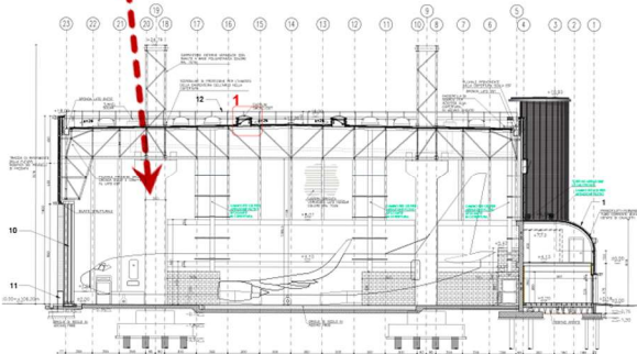
SECTION WITH IDENTIFICATION OF WASHED OUT WALLS
