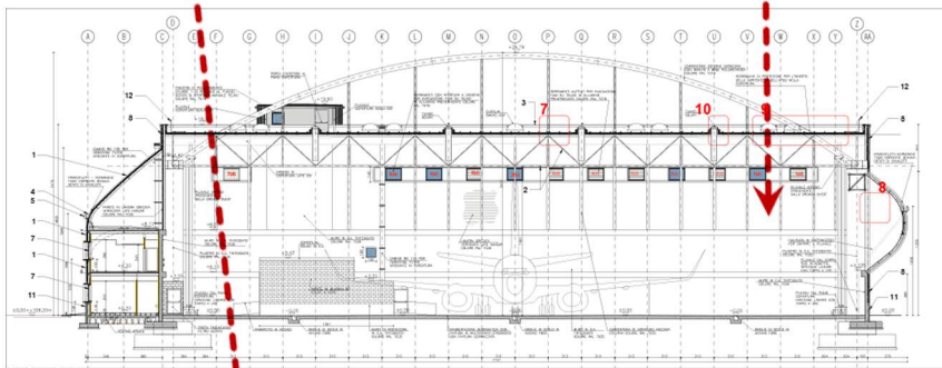
SECTION WITH IDENTIFICATION OF WASHED OUT WALLS
